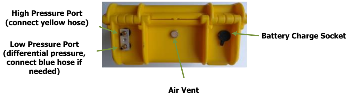
Figure 9 - CONNECTING TUBES
